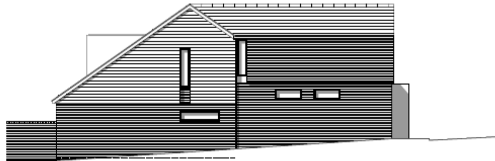
South Elevation
